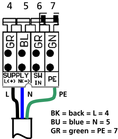
Illustration 4: Configuration terminals 4, 5, 7
