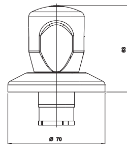
590 00 025 Final Assembly Set Assembly kit 2 with handle unit
